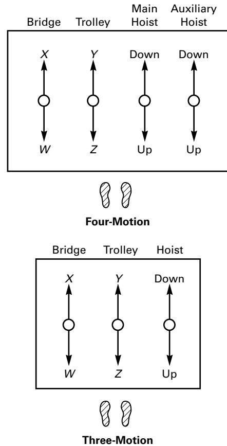
Fig. 2-1.13.3-4 Recommended Arrangement of Controllers (Radio Crane Control Transmitter Lever Arrangement)
